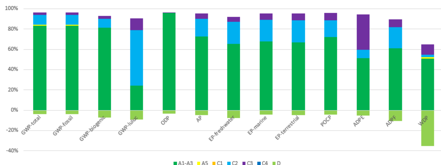
Dominance analysis
